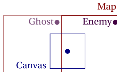
Figure 3: Finding the nearest "ghost" in all clones of the map. Here the player is the blue dot at the canvas center, and the enemy at is at the top right corner of the map. Since the map is a torus, the quickest route to the enemy is by going left and up, toward the enemy "ghost". The player radar always indicates the nearest ghost rather than real map position.
